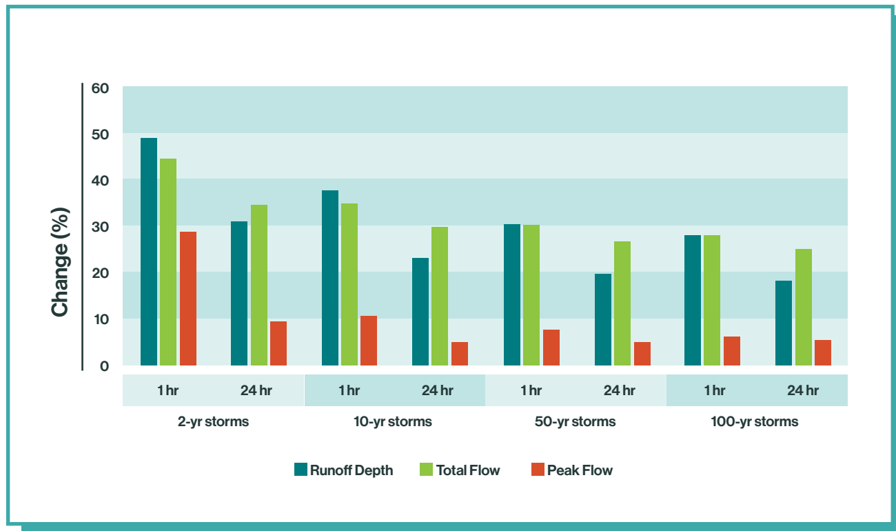
Figure 1. Flood risk reduction performance of distributed GSI (reducing effective impervious cover from 30% to 10%) and other BMPs in 185-acre Berry Brook watershed, Dover, NH
